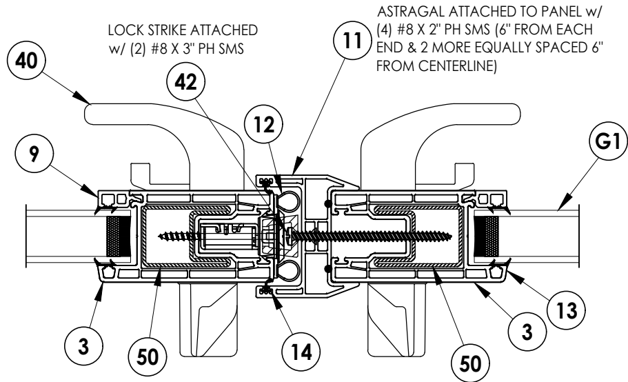
2 2 HORIZONTAL CROSS SECTION Shown w/ 1X Buck (Direct to Masonry Similar)
