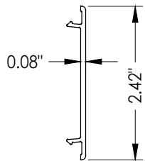
8 FRAME COVER
