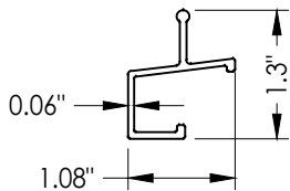
20 SILL CLADDING
