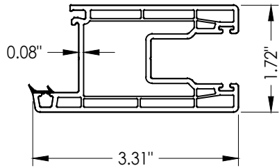
3 STILE & RAIL
