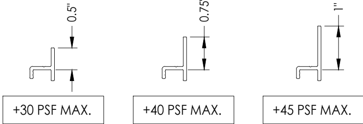
SILL RISER HEIGHT OPTIONS & DESIGN PRESSURE LIMITATIONS
