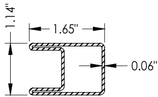
50 REINFORCEMENT Stile & Rail
