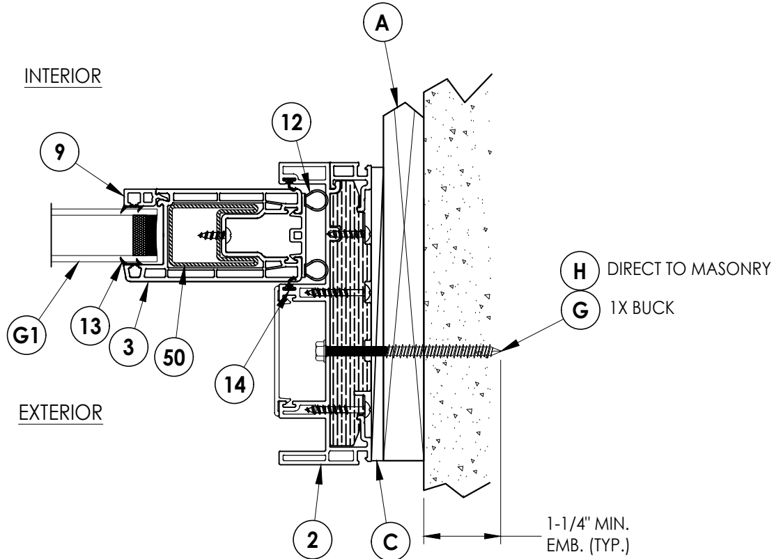
2 2 HORIZONTAL CROSS SECTION Shown w/ 1X Buck (Direct to Masonry Similar)
