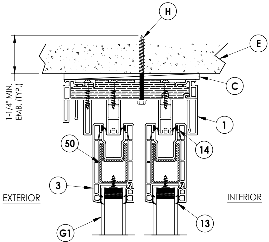
3 3 VERTICAL CROSS SECTION Shown Direct to Masonry
